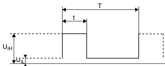
Fig. 49 Signal MLI
