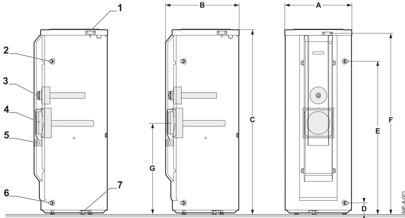
Fig.5 Dimensions
